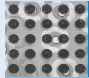
Voiding in a Micro BGA array.
