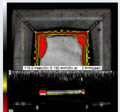
Q-BAM Cross Sectional View of Defect
