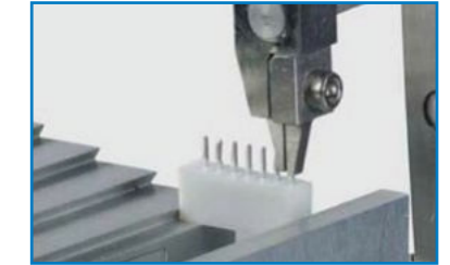
Torsion Testing
